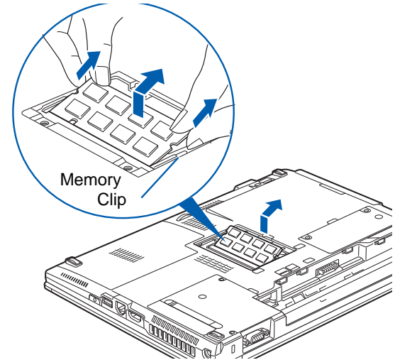
Figure 34. Removing memory module
