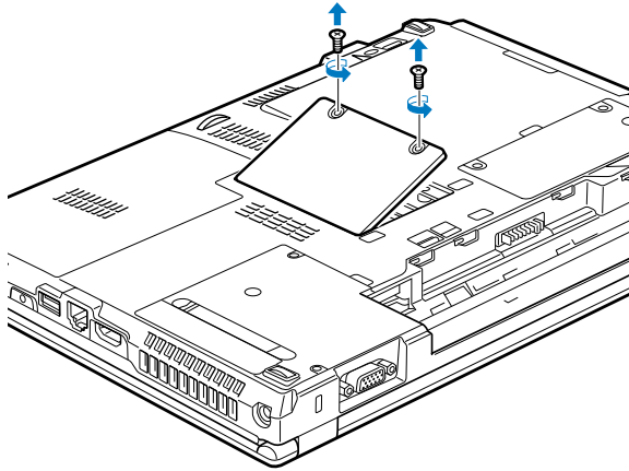
Figure 32. Opening the Memory Compartment
