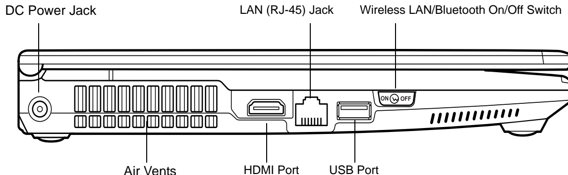
Figure 3. LifeBook notebook left-side panel
