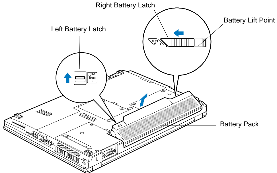
Figure 26. Removing a Battery
