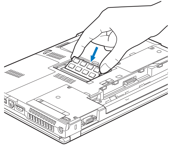
Figure 33. Installing a Memory Module
