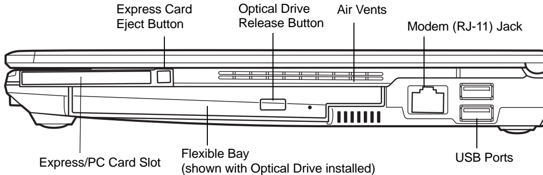
Figure 4. LifeBook notebook right-side panel
