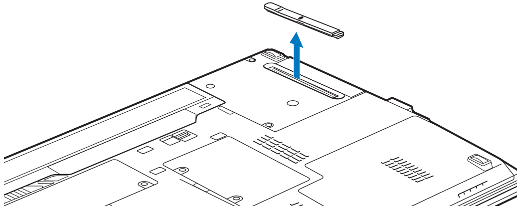
Figure 40. Retrait/installation du filtre anti-poussière
